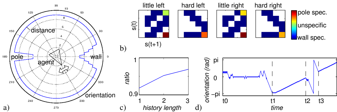
Fig. 3. a) Computer simulation of an agent that can change its orientation and measure distance. b) History length 1 SMCs ( p^1 ) emerging from learning after 10,000 iterations in an arena containing a pole and a wall. The plots show the conditional probabilities of observing distance sensor reading s(t+1) after executing the action given at the top of each panel, when the current distance reading is s(t) . Action-observation tuples (SMCs) in red/blue are exclusively observed when focusing the pole/wall, other colors are less specific, white patches represent tuples that have never been observed. c) Ratio of SMCs that are specific for one of the two objects for each of the three history lengths used. The ratio of object-specific SMCs increases with history length. d) Plot of the agent’s orientation over time in an experiment showing object-following behavior. After associating a reward with the SMCs of the pole for some time, the agent is initialized to a random orientation at t_0 . It starts moving randomly, eventually getting sight of the pole located at orientation -\pi at t_1 . Then the pole starts moving counter-clockwise, and the agent maintains focus. At t_2 the pole is in front of the wall (having identical distance), and the agent loses track. However, it quickly reorients and continues following at t_3 .
