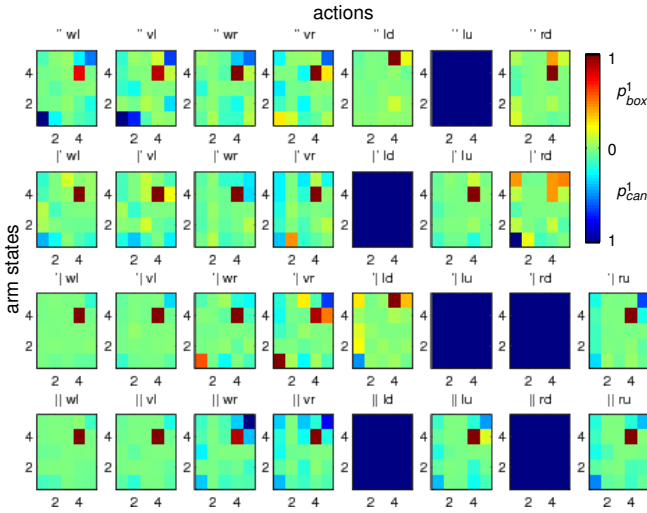
Fig. 4. SMCs of a can (cold colors) and a box (warm colors) for history length 1 ( p_o^1 ). Columns correspond to 8 possible actions, rows to 4 possible states of the 2 arms. Each plot gives the probability of observing s(t+1) (x-axis) given s(t) (y-axis). Note how the flat face of the box generates a high probability of repeatedly observing sensor value 4, and how the can generates several different contexts. Empty plots correspond to impossible actions.
