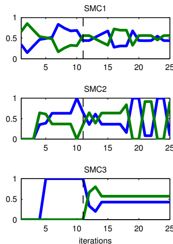
Fig. 5. To test the capabilities for object recognition by exercising its acquired SMCs, we present the robot with one of the two learned objects and record the conditional probabilities for each object over time (blue: can, green: box). After 10 iterations the objects are exchanged (dashed line). Note how increasing history length (SMC1→SMC2→SMC3) leads to a more and more sustained larger probability for the correct object identity, hence showing evidence for object-related SMCs.
