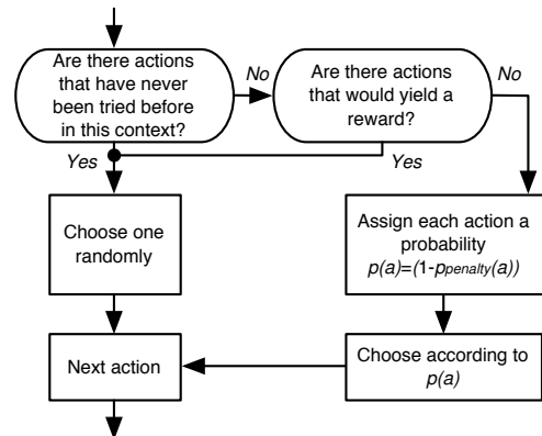
Fig. 2. Schematic of the action selection algorithm based on rewards observed in the past.
